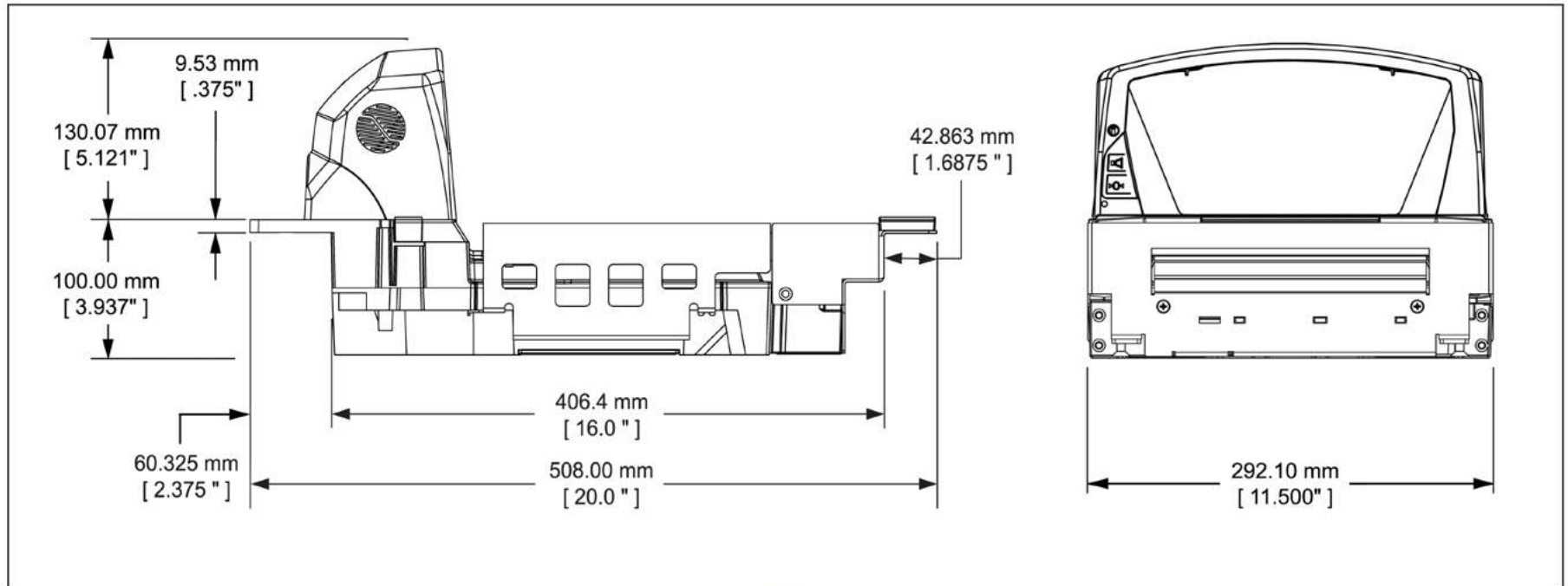
Figure 8. MS2430 Dimensions
